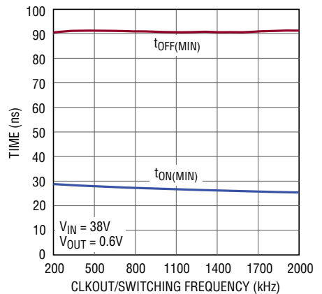
t ON(MIN) and t OFF(MIN) vs Switching Frequency
